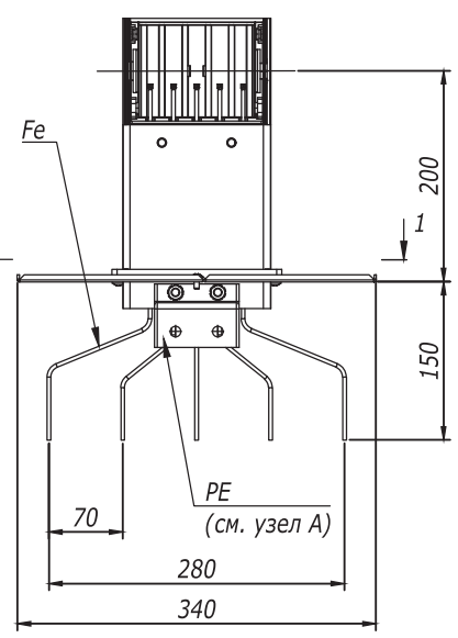
3P+N+PE+FE
